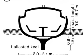
15 Keel cruiser: section
